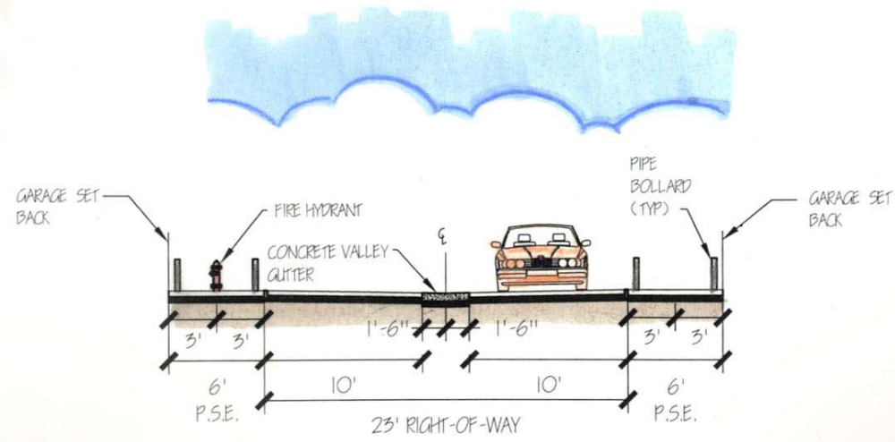
ALLEY FOR REAR LOADED RESIDENTIAL USE
